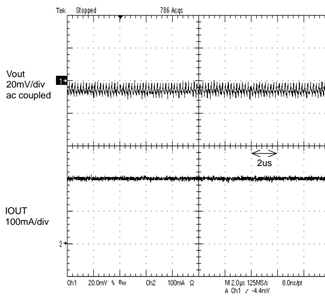
Figure 14. PWM mode Operation Iout=200mA
