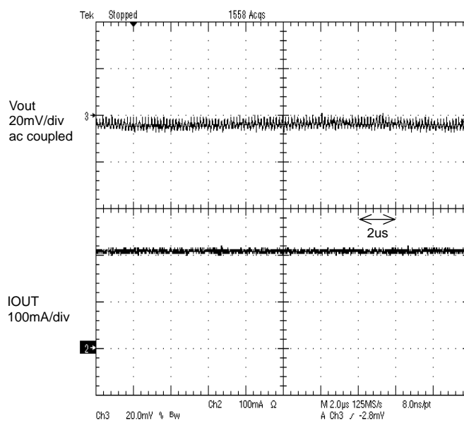
Figure 30. PWM mode Operation Iout=200mA
