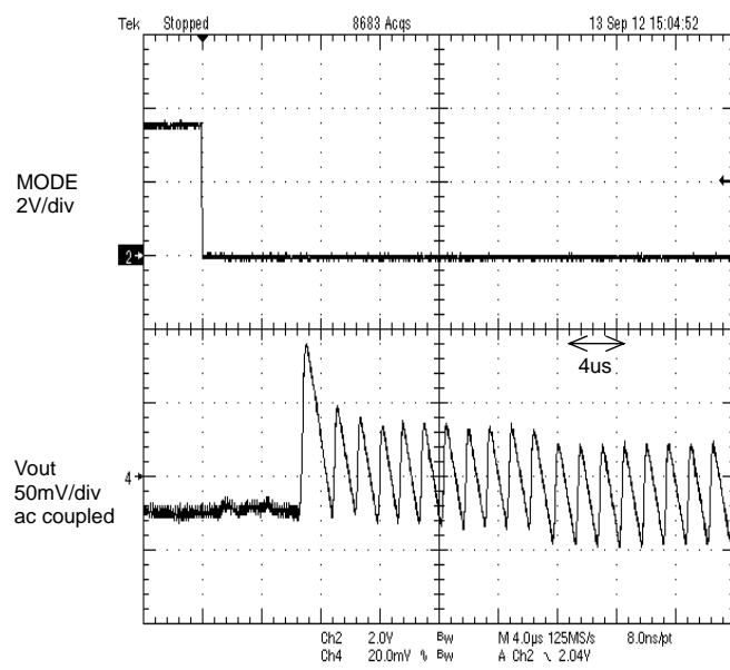
Figure 48. Mode Change Response MODE : High to Low
