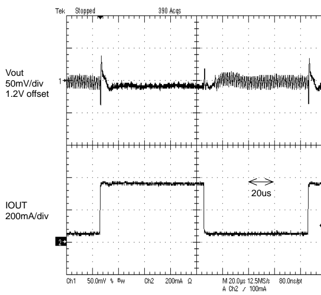
Figure 8. Load transient response 50mA to 350mA t_r=t_f=100\text{ns} , MODE : Low
