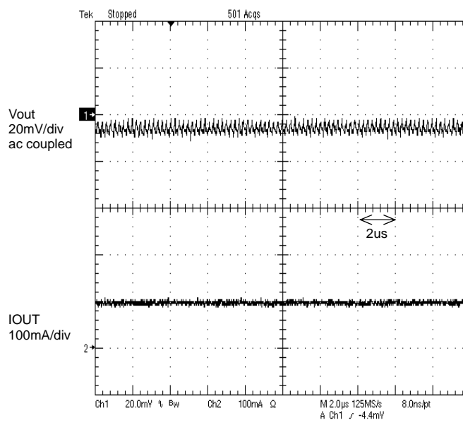
Figure 12. PWM mode Operation Iout=100mA
