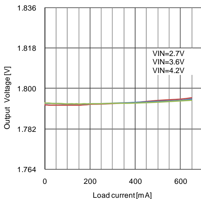
Figure 36. Load regulation PWM mode
