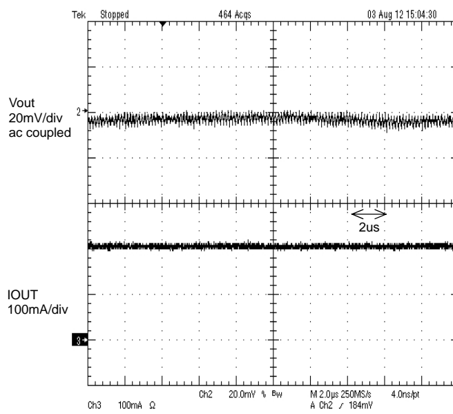
Figure 46. PWM mode Operation Iout=200mA
