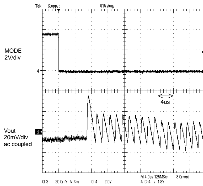
Figure 32. Mode Change Response MODE : High to Low
