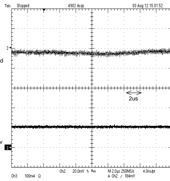
Figure 44. PWM mode Operation Iout=100mA
