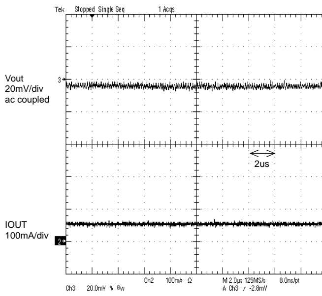
Figure 26. PWM mode Operation Iout=50mA
