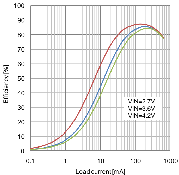
Figure 34. Efficiency vs Load current PWM mode
