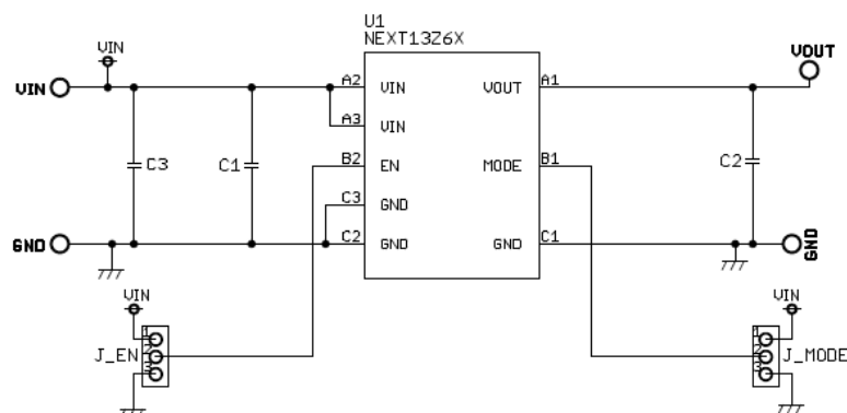
Figure 56. PCB Circuit
