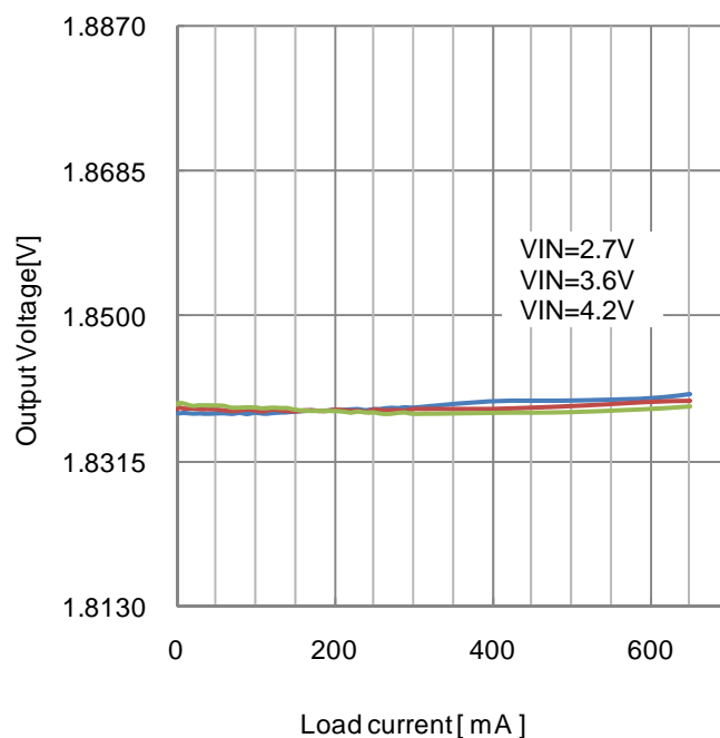
Figure 52. Load regulation PWM mode
