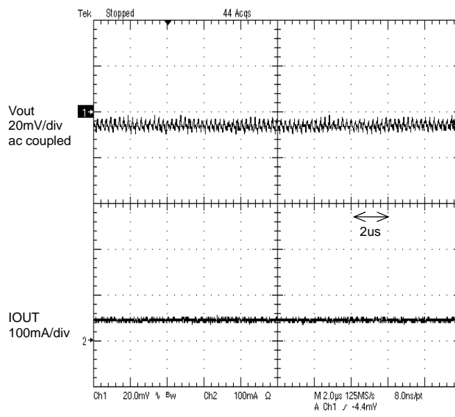
Figure 10. PWM mode Operation Iout=50mA
