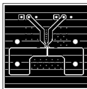
Figure 55. PCB layout (solder side)
