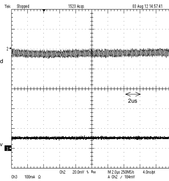
Figure 42. PWM mode Operation Iout=50mA
