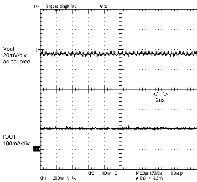
Figure 28. PWM mode Operation Iout=100mA
