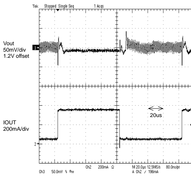
Figure 24. Load transient response 50mA to 350mA t_r=t_f=100\text{ns} , MODE : Low
