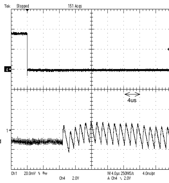
Figure 16. Mode Change Response MODE : High to Low
